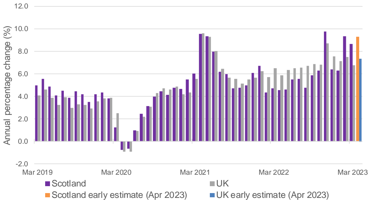
Chart 10: Annual Percentage Change in Median Monthly Pay, Scotland and UK, March 2019 to April 2023
