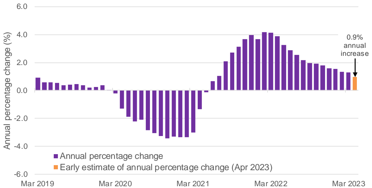
Chart 8: Annual Percentage Change in Payrolled Employees, Scotland, March 2019 to April 2023
