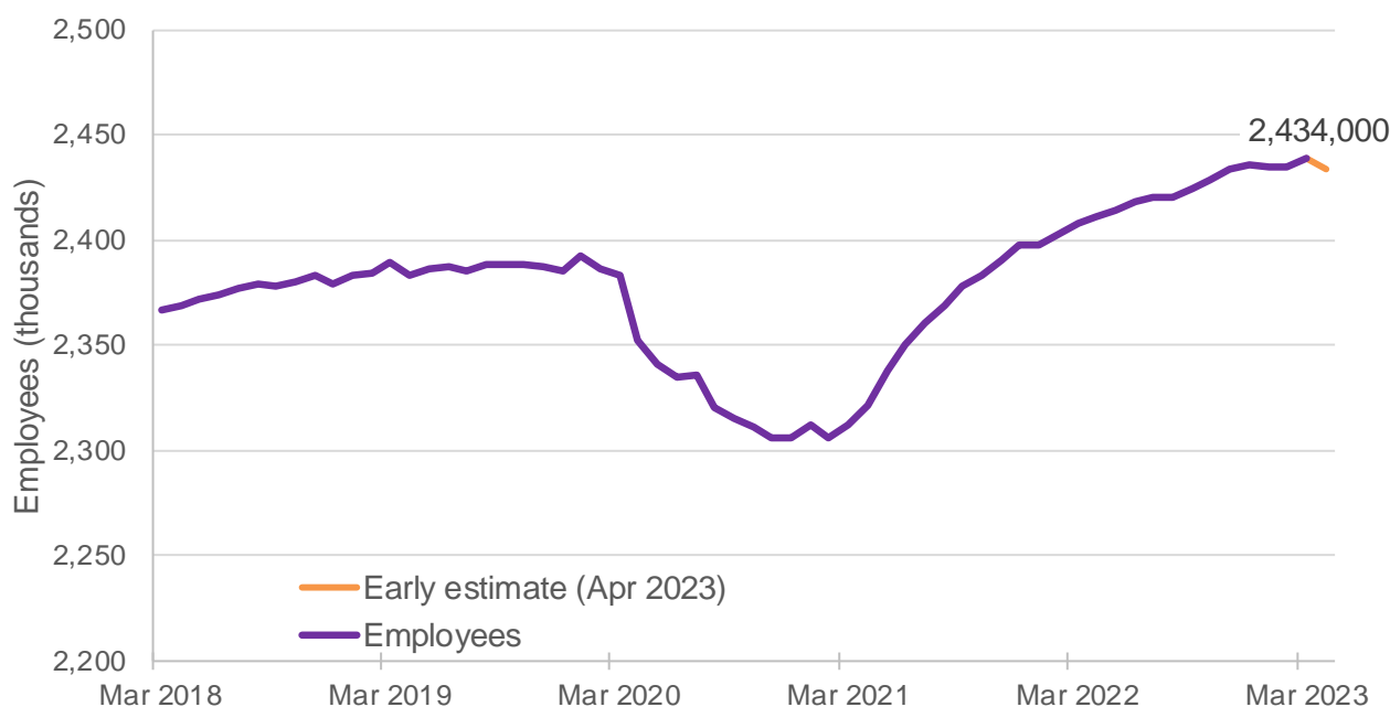
Chart 7: Payrolled Employees, Scotland, March 2018 to April 2023, seasonally adjusted
