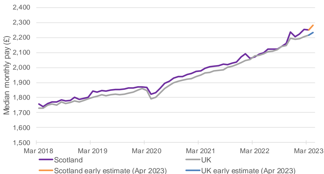
Chart 9: Median Monthly Pay, Scotland and UK, March 2018 to April 2023, seasonally adjusted
